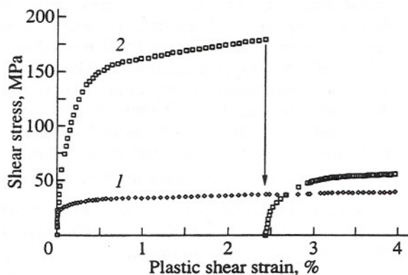
Fig. 4. Resolved shear stress plotted against shear strain in \text{Ni}_3\text{Al} : (1) at 300 K; (2) at 875 K (at the first stage) and 300 K (at the second stage) [4].
