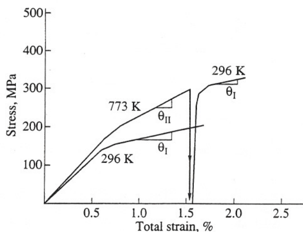
Fig. 3. Stress-strain curves for TiAl single crystals. Lower curve, compression at room temperature; upper curves, two-stage straining [3].
