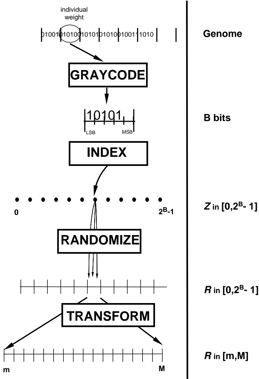
Figure 1: Encoding weights
